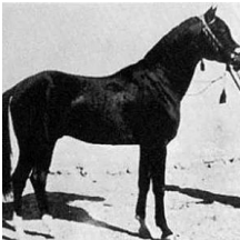
Gabor 1944 Black
